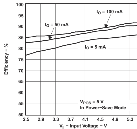
图 8-14. TPS65130 Efficiency vs Input Voltage
