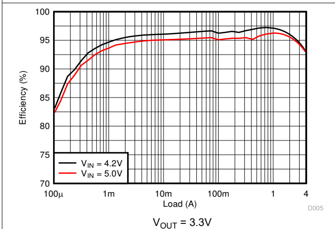
图 8-19. Efficiency
