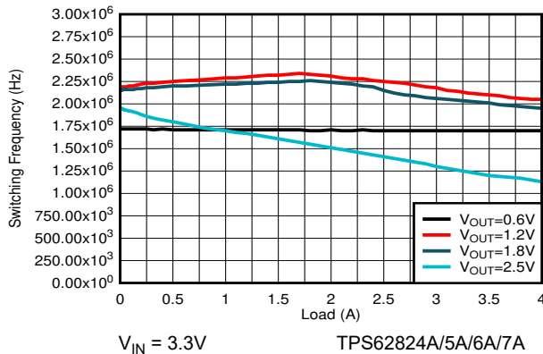
图 8-25. Switching Frequency
