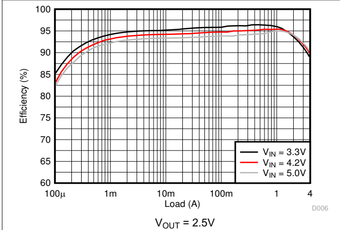
图 8-15. Efficiency
