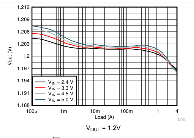
图 8-8. Load Regulation
