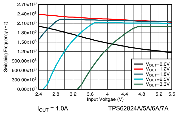
图 8-26. Switching Frequency
