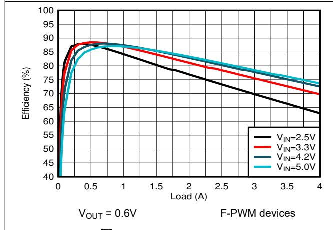
图 8-5. PWM Efficiency
