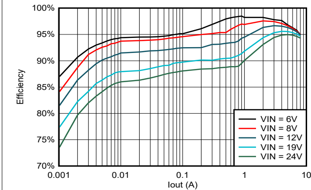
图 5-17. TPS56837 效率, V_{out} = 5V , F_{sw} = 500kHz
