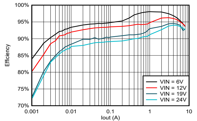
图 5-18. TPS56837 效率, V_{out} = 5V , F_{sw} = 800kHz
