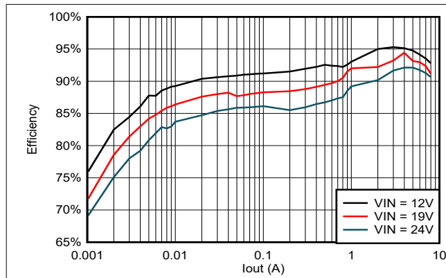
图 5-19. TPS56837 效率, V_{out} = 5V , F_{sw} = 1200kHz
