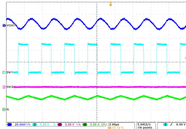
图 8-2. Switching Waveforms in V_{IN} = 12\text{ V} , V_{OUT} = 5\text{ V} , I_O = 5\text{ A} , FPWM
