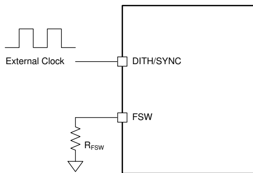
图 7-3. External Clock Configuration
