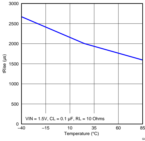
Figure 20. Rise Time vs Temperature
