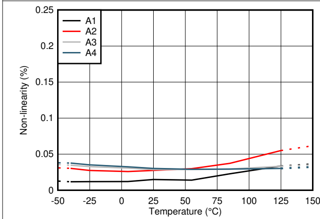
图 7-3. Non-Linearity vs. Temperature
