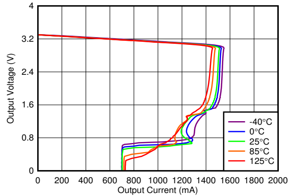
图 5-26. I_{OUT} vs V_{OUT} Pulldown Resistor
