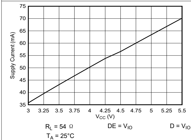
图 6-3. Supply Current vs Supply Voltage
