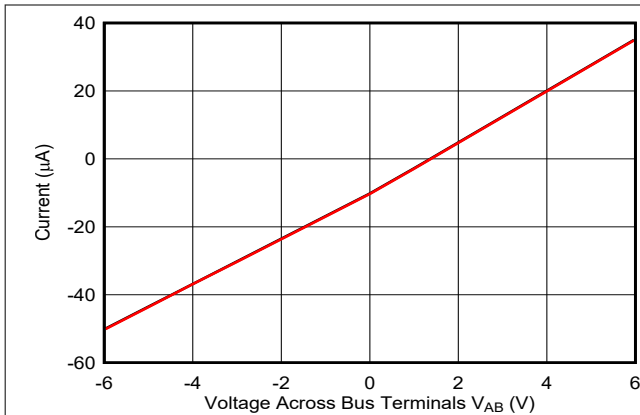
图 8-3. Voltage vs Current Across AB Bus Pins with Termination OFF
