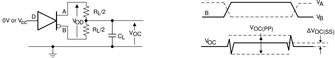
图 7-2. Measurement of Driver Differential and Common-Mode Output With RS-485 Load
