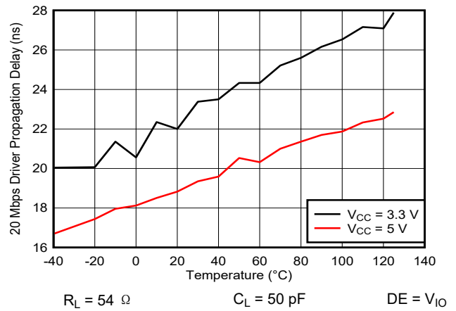
图 6-8. Driver Propagation Delay vs Temperature (20 Mbps)
