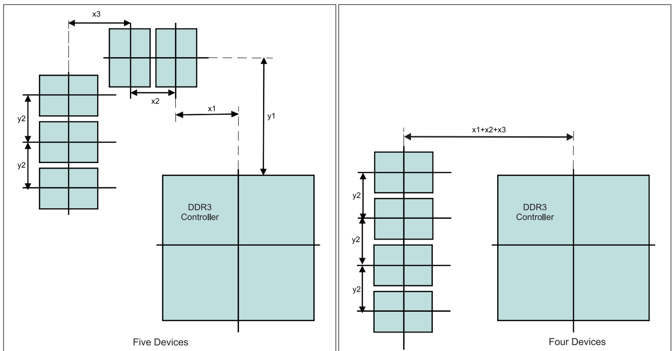
图 8-39. Placement Specifications
