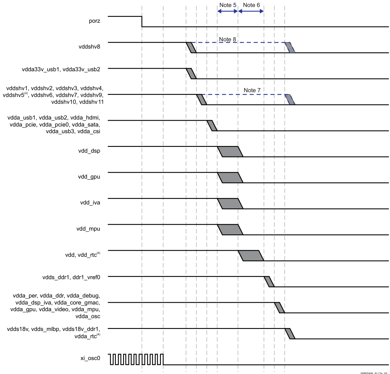
图 5-6. Power-Down Sequencing
