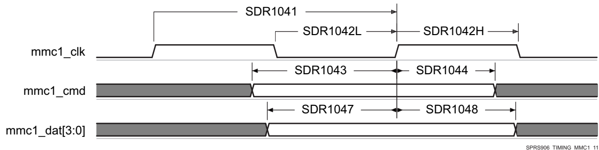
图 7-64. MMC/SD/SDIO in - High Speed SDR104 - Receiver Mode
