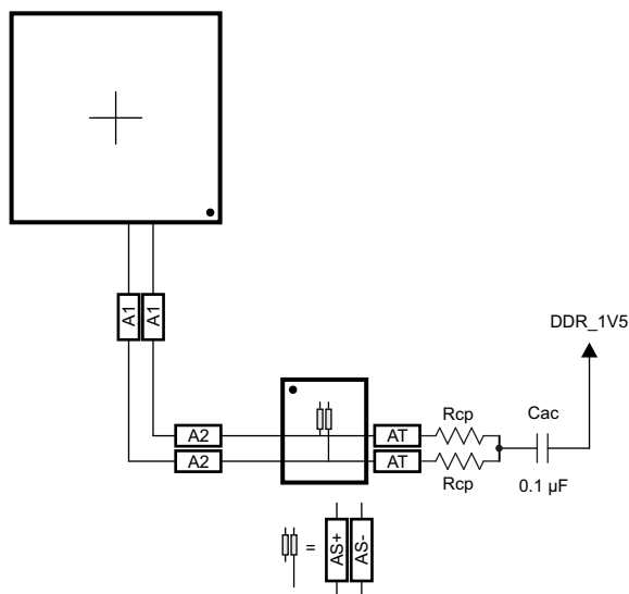
图 8-55. CK Routing for One DDR3 Device
