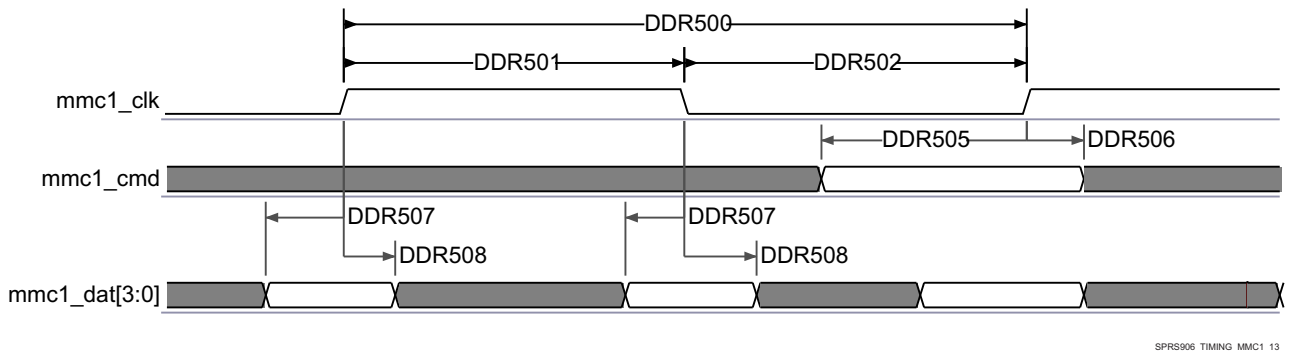
图 7-66. SDRAMC - High Speed SD - DDR - Data/Command Receive
