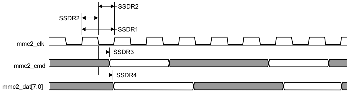
图 7-69. MMC/SD/SDIO in - Standard JC64 - Transmitter Mode
