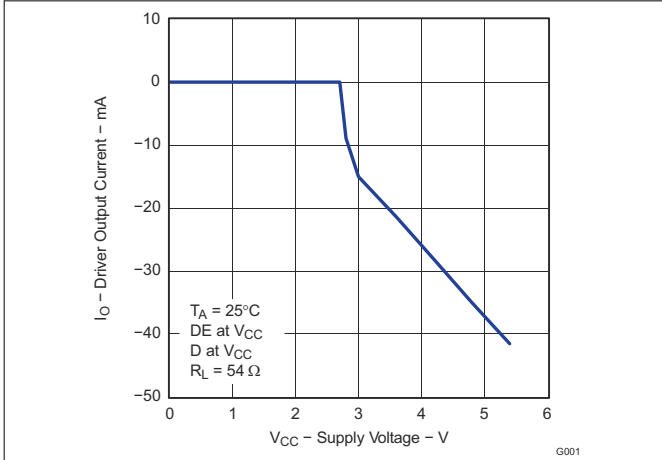
图 6-1. Driver Output Current vs Supply Voltage
