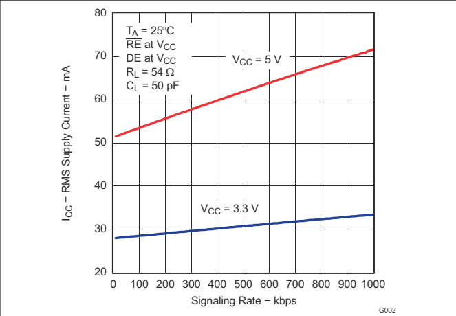
图 6-2. RMS Supply Current vs Signaling Rate
