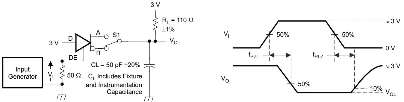
图 7-5. Measurement of Driver Enable and Disable Times With Active-Low Output and Pullup Load
