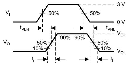
图 7-6. Measurement of Receiver Output Rise and Fall Times and Propagation Delays
