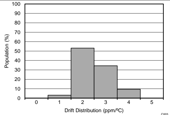
Figure 2. Drift Distribution
