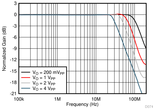
See 图 9-1, gain = 1\text{ V/V} , R_F = 0\ \Omega
