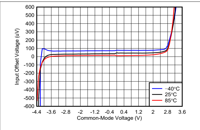
图 6-20. Input offset voltage vs Common-Mode Input Voltage
