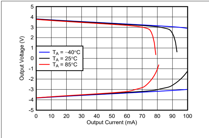
图 6-25. Output voltage vs Output Current Over Temperature
