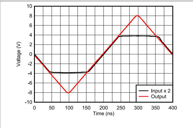
图 6-26. Noninverting Input Overdrive Recovery
