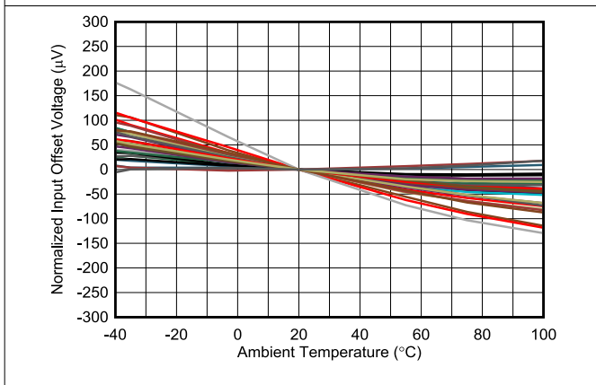
图 6-21. Typical Input Offset Voltage Over Temperature
