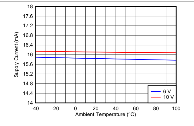
图 6-24. Supply Current vs Temperature
