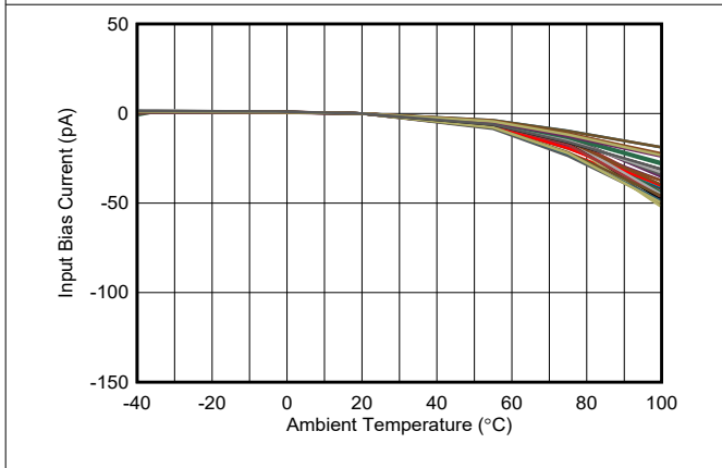
图 6-23. Typical Input Bias Current Over Temperature
