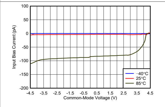
图 6-22. Typical Input Bias Current vs Common-Mode Input Voltage
