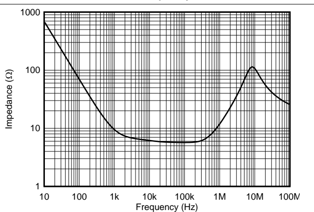
图 9. High-Drive Mode Open-Loop Output Impedance vs Frequency
