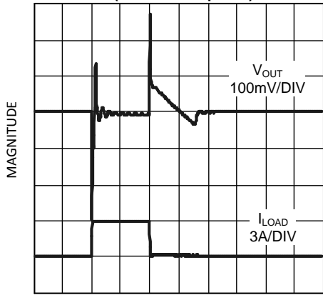
TIME (50 \mu\text{s}/\text{DIV} ) Figure 25.
