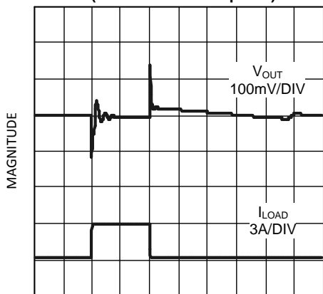
TIME (50 \mu\text{s}/\text{DIV} ) Figure 23.
