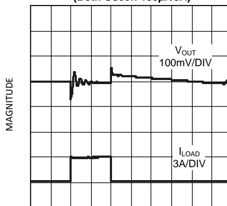
TIME (50 \mu\text{s}/\text{DIV} ) Figure 22.
