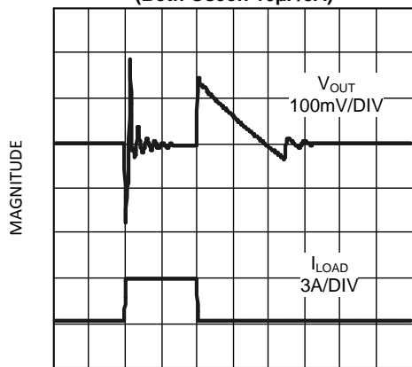
TIME (50 \mu\text{s}/\text{DIV} ) Figure 21.
