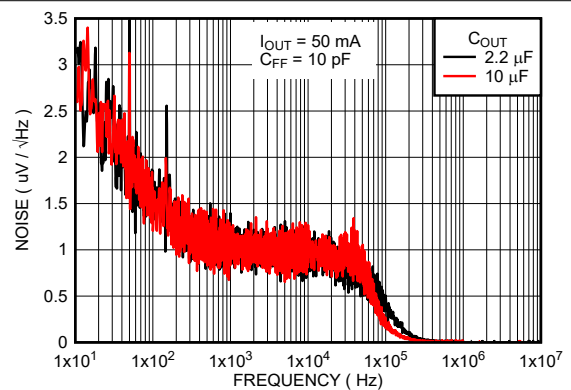
图 6-34. Output Noise Density for Legacy Chip
