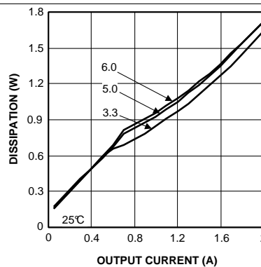
Figure 10. Dissipation 42-V Input
