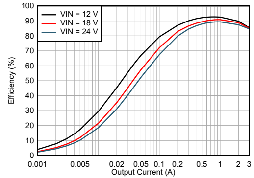
LMQ66430MC3 V_{OUT} = 3.3V 2.2MHz (FPWM) 修复
