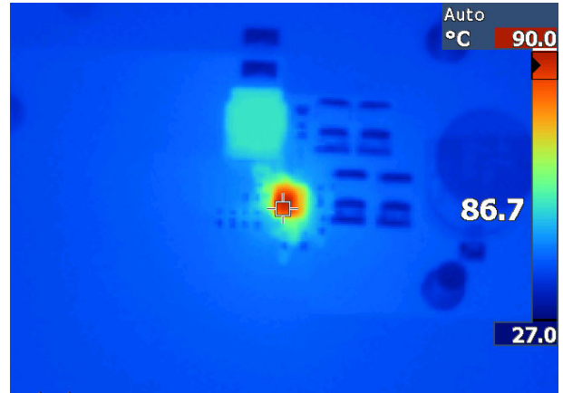
LMQ66430MC3 V_{OUT} = 3.3V 12V_{IN} , 3A, 2.2MHz 修复
