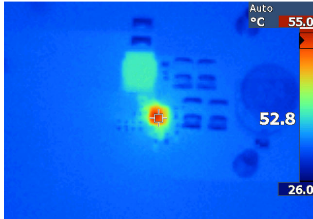
LMQ66430MC3 V_{OUT} = 3.3V 12V_{IN} , 2A, 2.2MHz 修复
