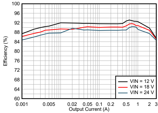
LMQ66430MC3 V_{OUT} = 3.3V 2.2MHz (自动) 修复
