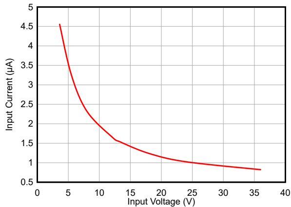
LMQ66430MC3 V_{OUT} = 3.3V 2.2MHz (自动) 修复 空载
