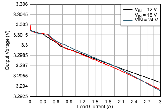
LMQ66430MC3 V_{OUT} = 3.3V 2.2MHz (自动) 修复
