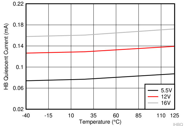
图 6-3. HB Quiescent Current
