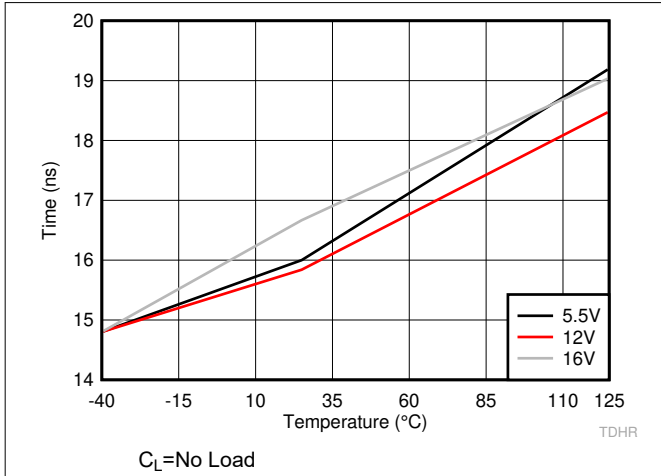
图 6-20. HO Rising Propagation Delay (TDHRR)
