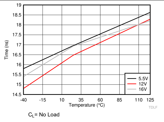
图 6-23. LO Falling Propagation Delay (TDLFF)
