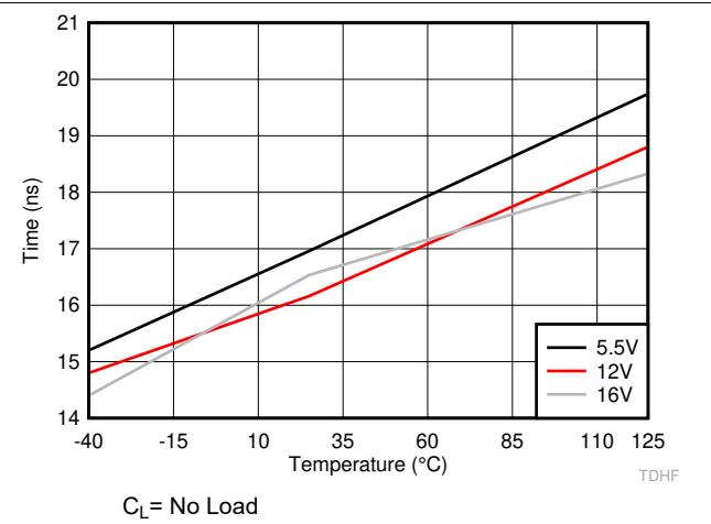
图 6-21. HO Falling Propagation Delay (TDHFF)
