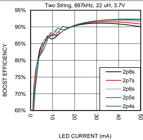
图 38. Boost Efficiency vs Series LEDs
