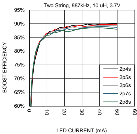
图 40. Boost Efficiency vs Series LEDs
