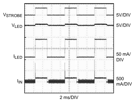
Figure 34. Assist PWM
