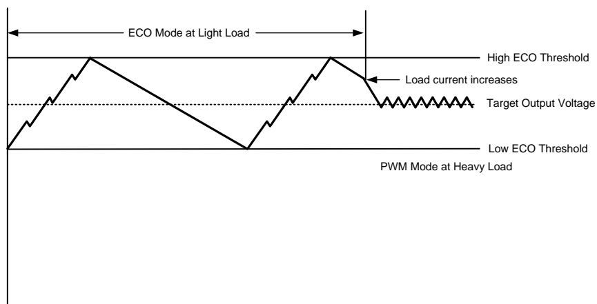
Figure 23. Operation in ECO Mode and Transfer to PWM Mode
