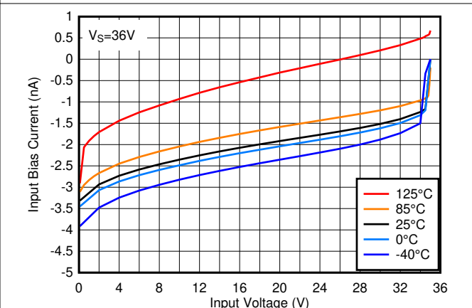
图 6-18. Input Bias Current vs. Input Voltage at 36V
