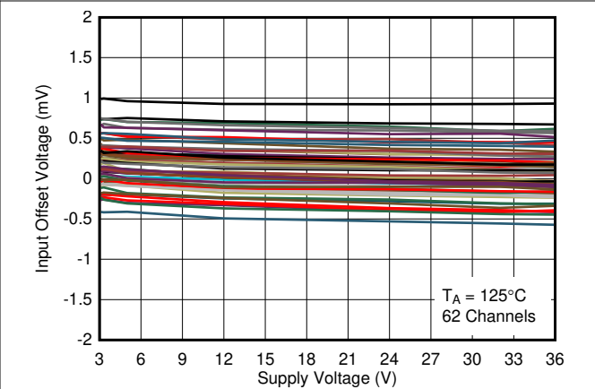
图 6-14. Input Offset Voltage vs. Supply Voltage at 125°C
