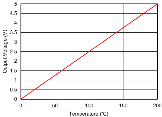
图 9-9. Transfer Function of a 3-Wire RTD Interface
