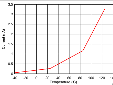
D007_Leakage.grf
