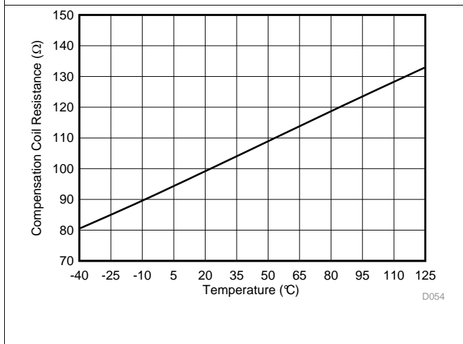
图 17. Compensation Coil Resistance vs Temperature
