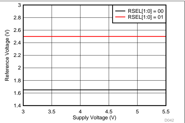
图 50. Reference Voltage vs Supply Voltage
