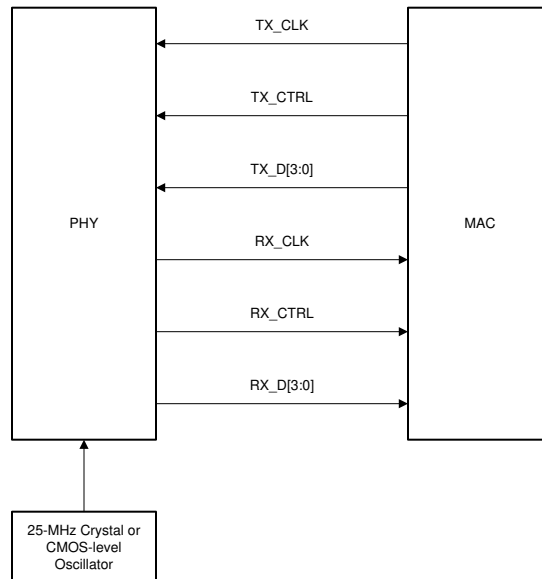
图 7-16. RGMI Connections
