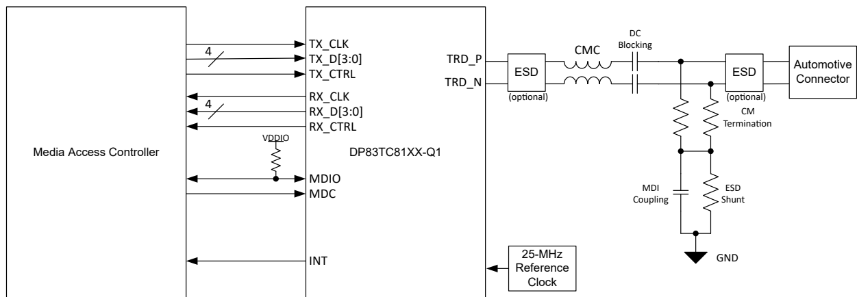
图 8-5. Typical Application (RGMII)
