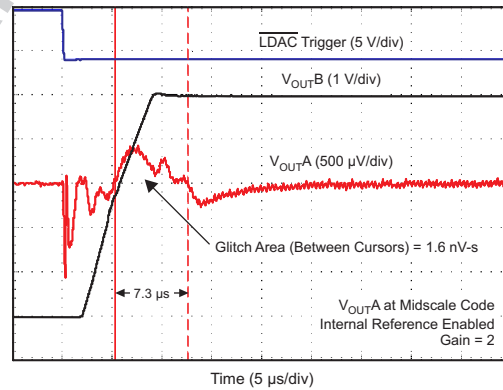
图 43. Channel-to-Channel Crosstalk 5-V Rising Edge
