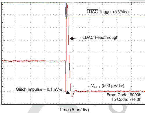
图 42. Glitch Impulse Falling Edge, 16-LSB Step
