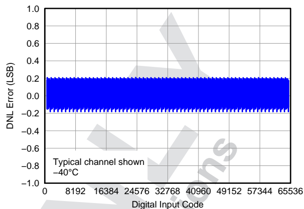
图 56. Differential Linearity Error vs Digital Input Code ( -40^\circ\text{C} )
