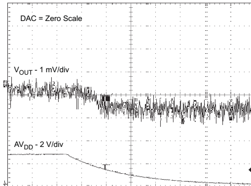
POWER-OFF GLITCH
