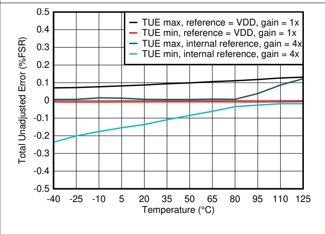
图 6-7. Total Unadjusted Error vs Temperature
