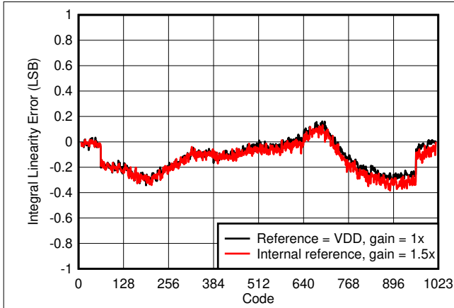
图 6-12. Integral Linearity Error vs Digital Input Code
