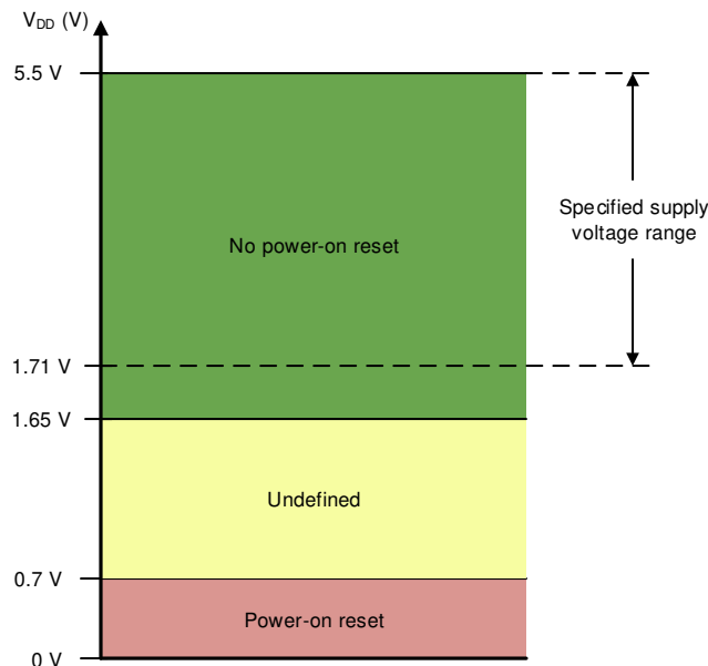
图 7-1. Threshold Levels for the V_{DD} POR Circuit
