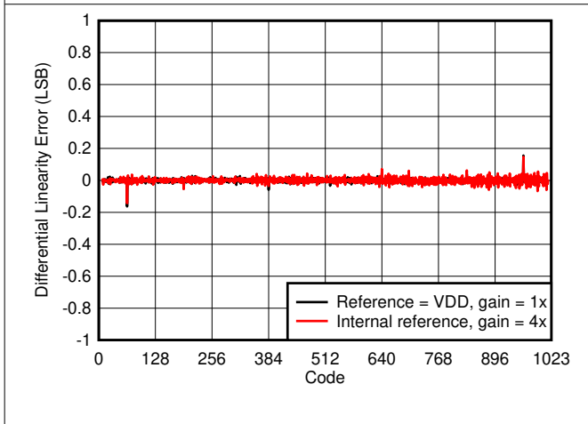
图 6-4. Differential Linearity Error vs Digital Input Code
