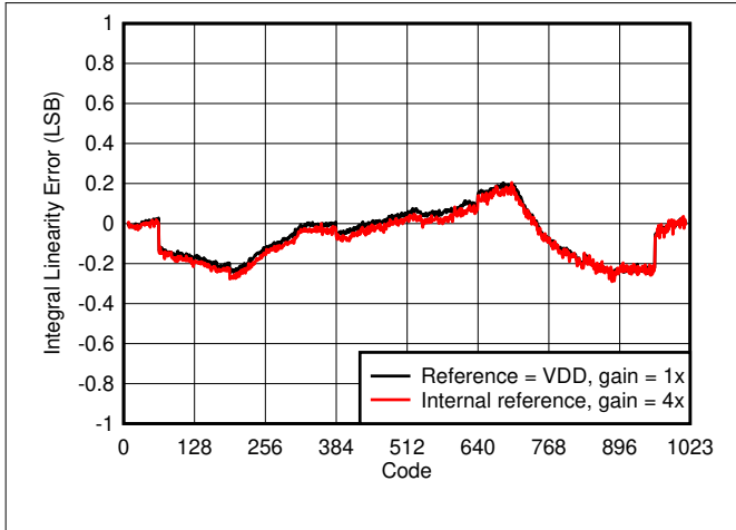
图 6-2. Integral Linearity Error vs Digital Input Code
