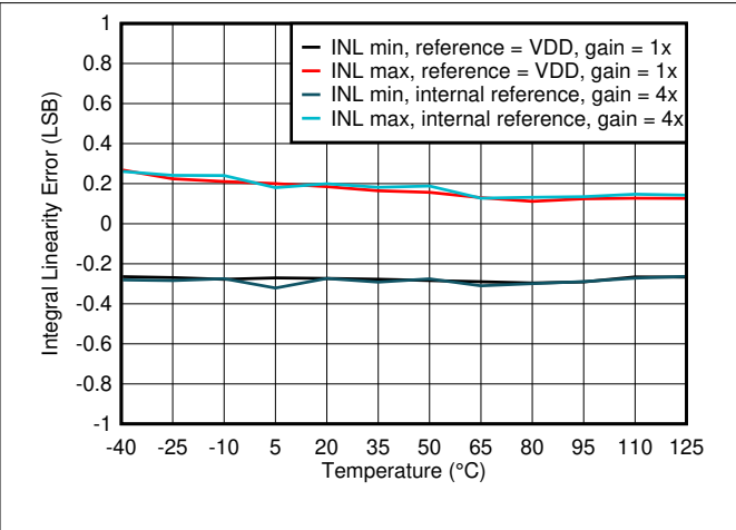
图 6-3. Integral Linearity Error vs Temperature
