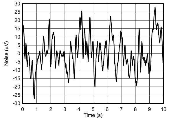
Internal reference (gain = 4 \times ), V_{DD} = 5.5\text{ V} , DAC at midscale
