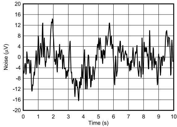
Reference = V_{DD} = 5.5\text{ V} , DAC at midscale
