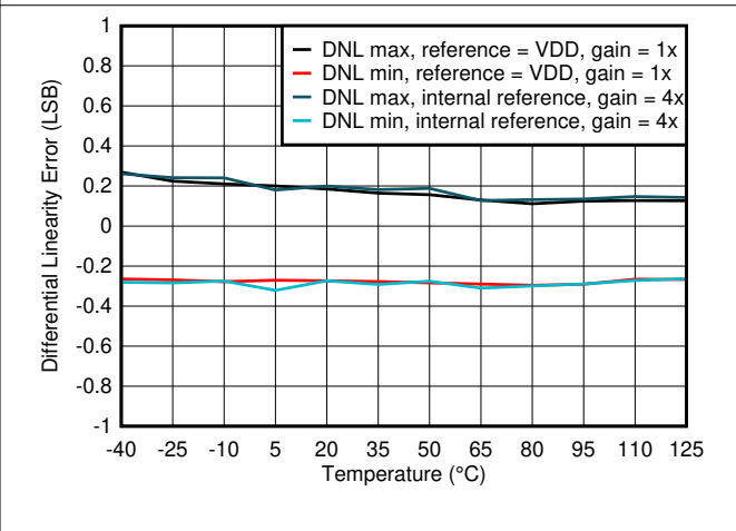
图 6-5. Differential Linearity Error vs Temperature
