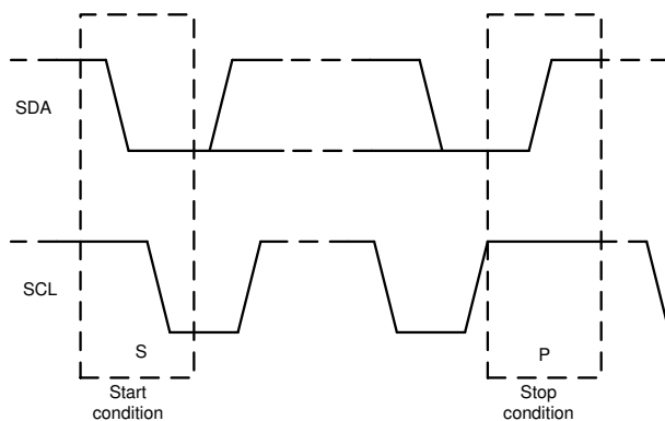
图 7-4. Start and Stop Conditions
