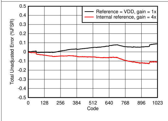
图 6-6. Total Unadjusted Error vs Digital Input Code
