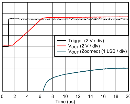
图 6-36. Glitch Impulse, Rising Edge, 1-LSB Step
