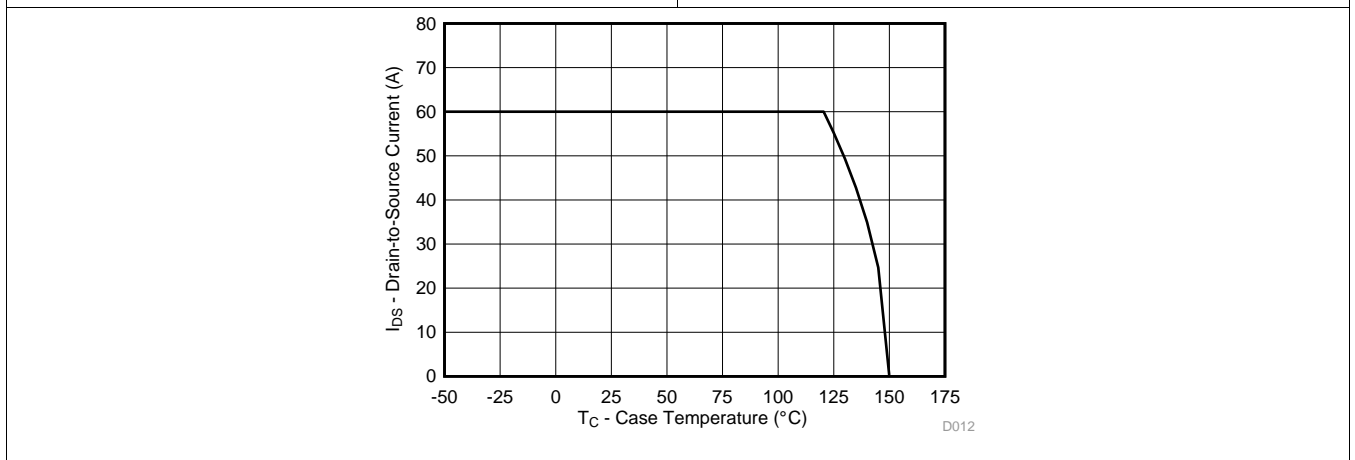
Figure 11. Single Pulse Unclamped Inductive Switching
