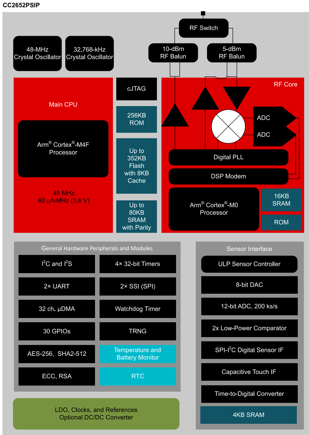
图 4-2. CC2652PSIP Hardware Overview
