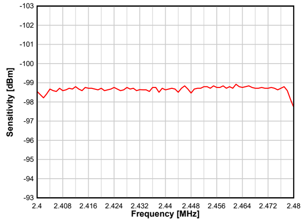
图 8-15. Sensitivity vs. Frequency (250 kbps)
