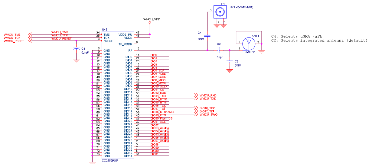
图 10-1. CC2652PSIP Typical Application Schematic
