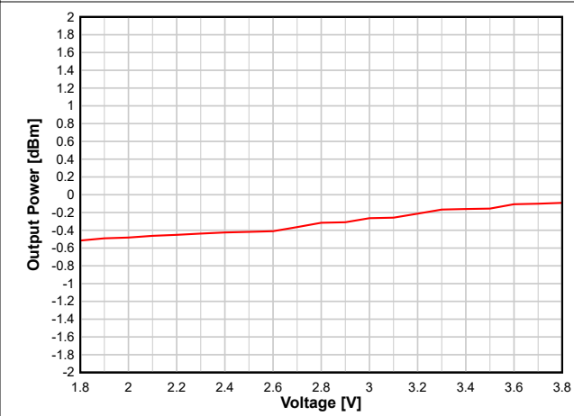
图 8-24. Output Power vs. Supply Voltage (VDD5) (BLE 1 Mbps, 2.44 GHz, 0 dBm)
