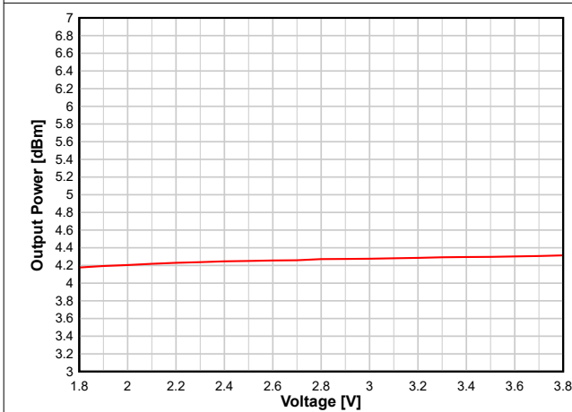
图 8-25. Output Power vs. Supply Voltage (VDD5) (BLE 1 Mbps, 2.44 GHz, +5 dBm)
