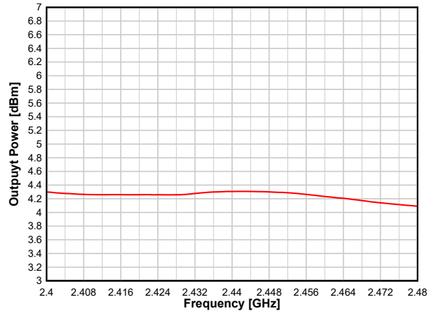
图 8-28. Output Power vs. Frequency (BLE 1 Mbps, +5 dBm)
