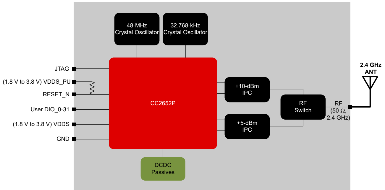
图 4-1. CC2652PSIP Block Diagram
