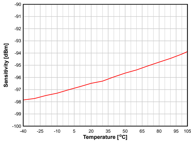
图 8-16. Sensitivity vs. Temperature (BLE 1 Mbps, 2.44 GHz)
