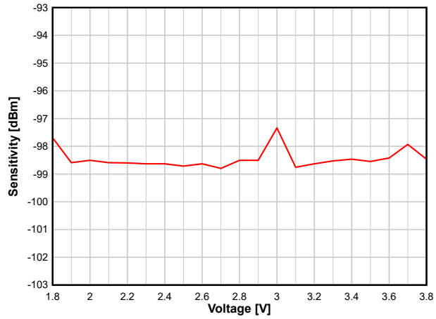
图 8-20. Sensitivity vs. Supply Voltage (VDD5) (250 kbps, 2.44 GHz)
