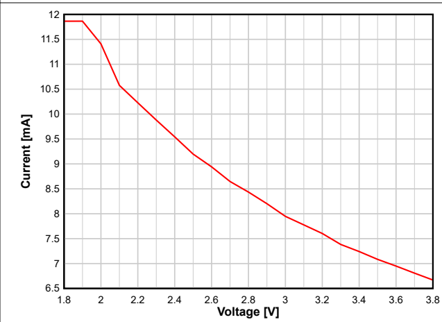
图 8-11. TX Current vs. Supply Voltage (VDD5) (BLE 1 Mbps, 2.44 GHz, 0 dBm)
