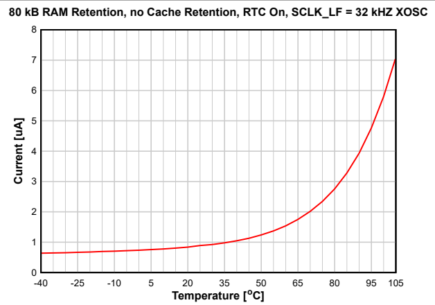
图 8-5. Standby Mode (MCU) Current vs. Temperature
