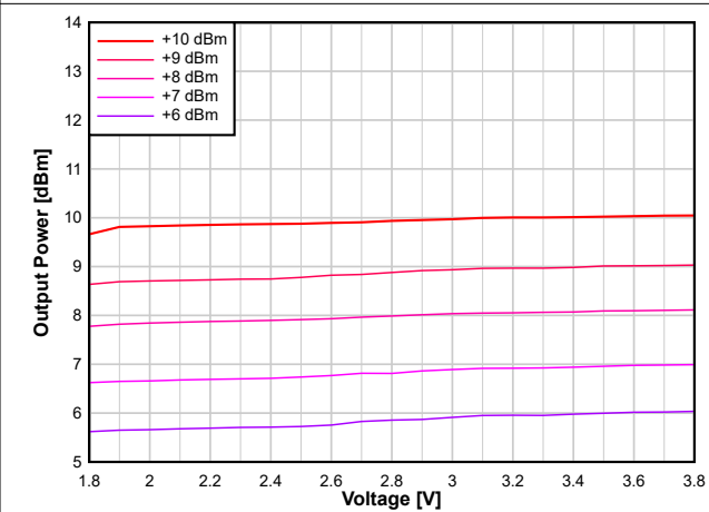
图 8-26. Output Power vs. Supply Voltage (VDD5) (2.44 GHz, +10 dBm PA)
