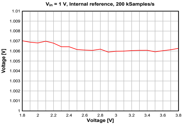
图 7-38. ADC Accuracy vs. Supply Voltage (VDD5)
