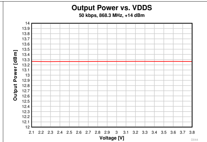
图 7-19. Output Power vs. Supply Voltage (VDD5) (50 kbps, 868.3 MHz)
