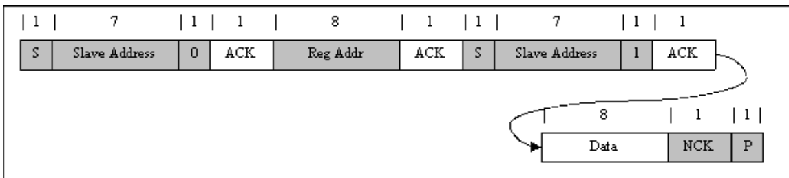
图 33. Single Read
