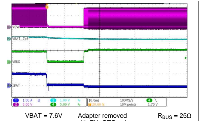
图 83. Buck Mode Startup After Adapter Removal
