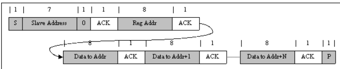
图 34. Multi-Write
