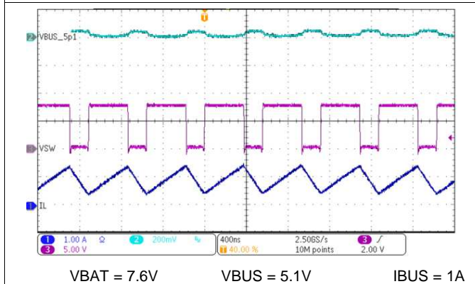
图 84. Buck Mode (OTG) PWM Switching
