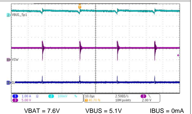
图 85. Buck Mode (OTG) PFM Switching
