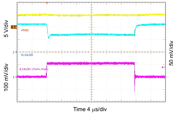
图 87. 1.2 V_{LSLDO} Load Transient, 0 to 100 mA
