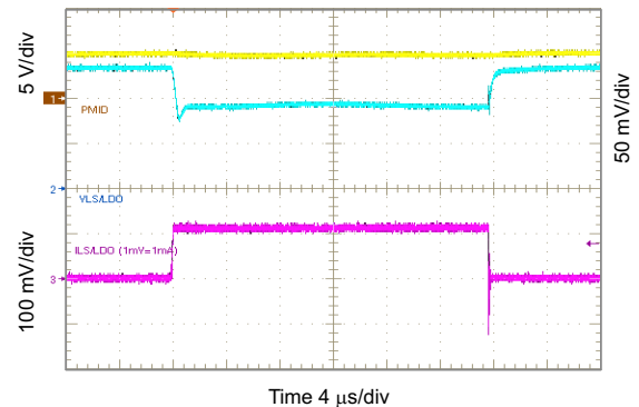
图 88. 1.8 V_{LSLDO} Load Transient, 0 to 100 mA
