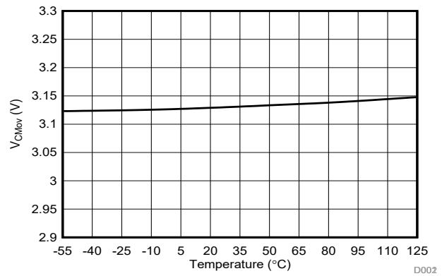
图 6-7. Common-Mode Overtolerance Detection Level vs Temperature
