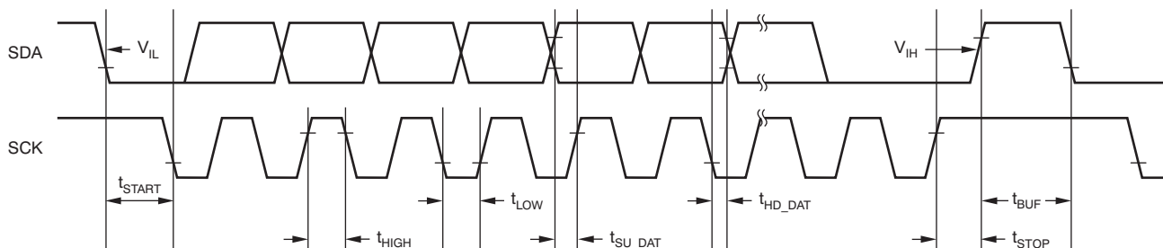
Figure 4. I 2 C Bus Interface Timing
