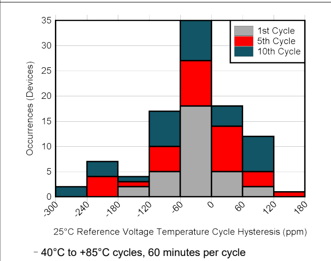
图 6-44. Multiple Temperature Cycle Hysteresis
