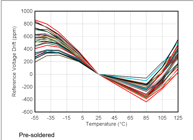
图 6-41. Reference Voltage Temperature Drift
