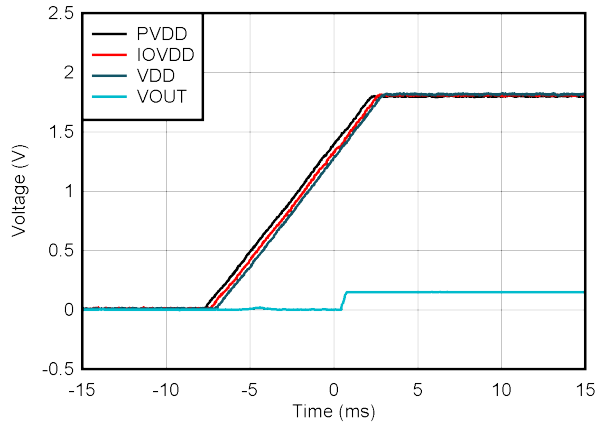
图 6-27. DAC Supply Power On, PVDD = 1.8 V
