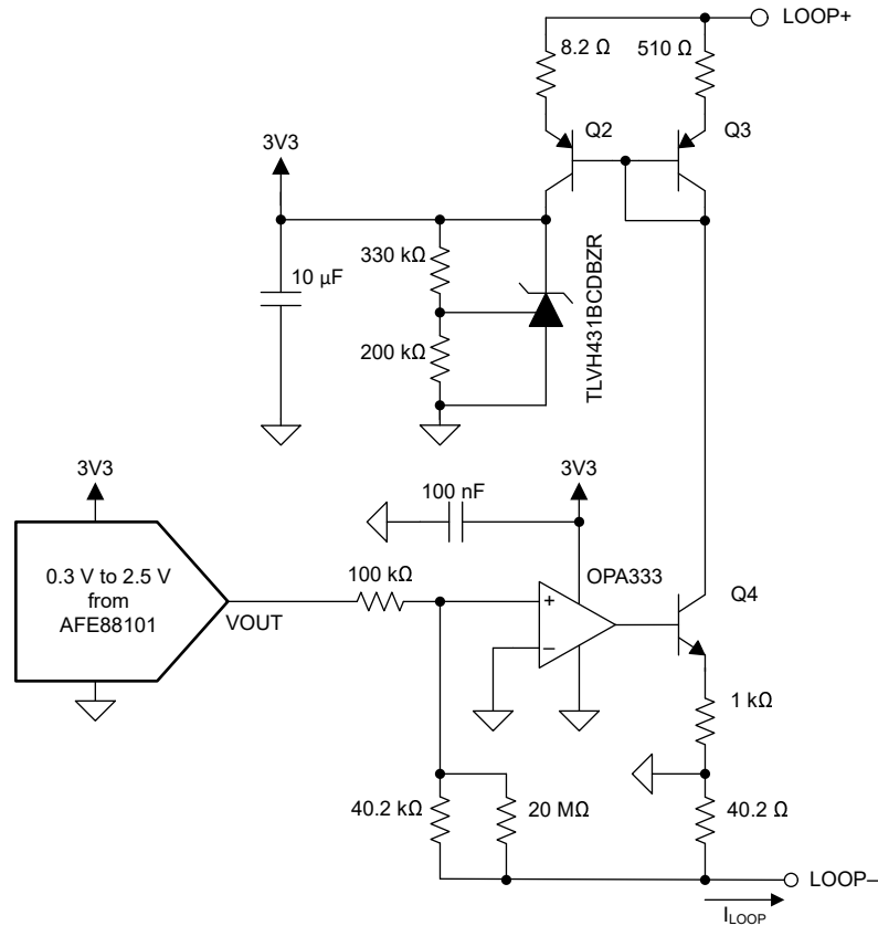
图 8-5. Current Loop Control for the AFE88101 Transmitter
