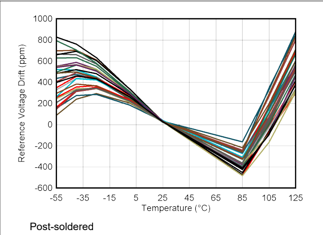
图 6-42. Reference Voltage Temperature Drift
