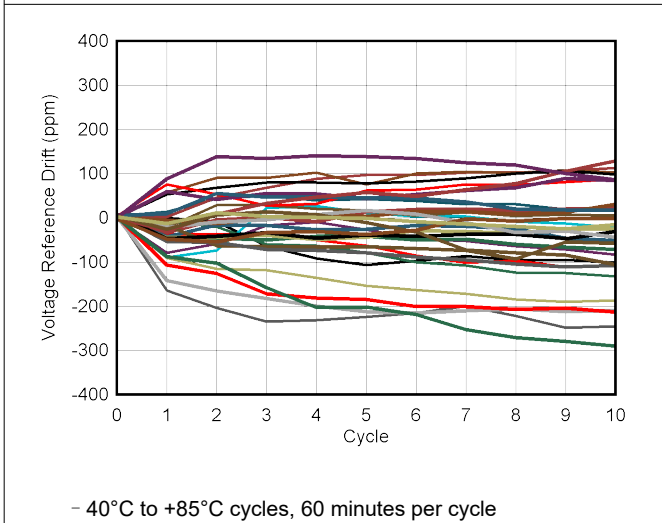
图 6-43. Multiple Temperature Cycle Hysteresis
