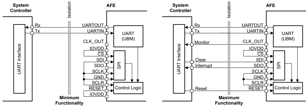
图 7-18. UBM (UART Interface) Connections
