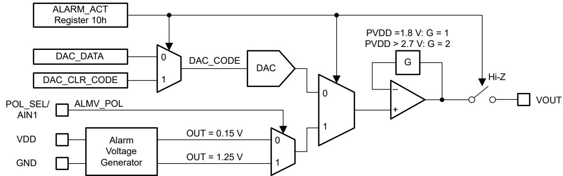
图 7-12. Alarm Voltage Generator Architecture
