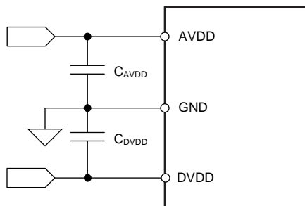
图 122. Power-Supply Decoupling
