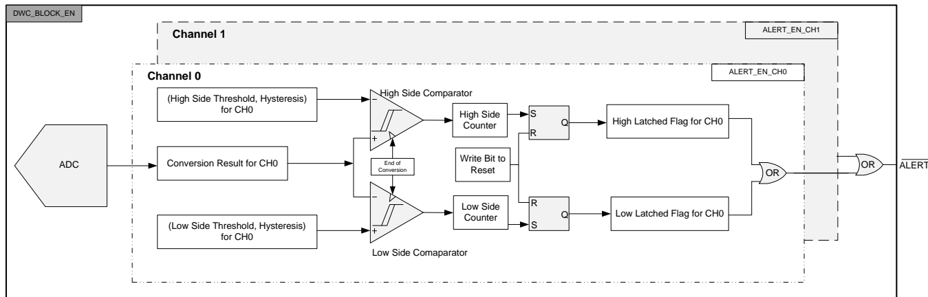
图 47. Digital Comparator Block Diagram
