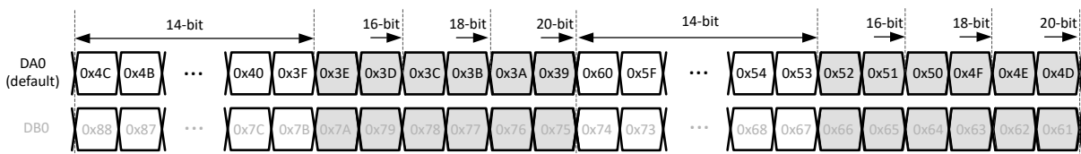
图 8-38. 1/2-wire output bit mapping
