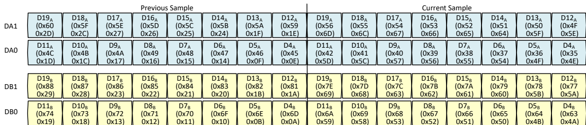
图 8-36. Example: 2-wire output bit mapping
