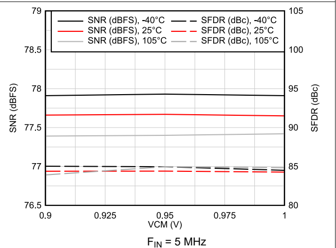
图 6-16. AC Performance vs VCM vs Temperature
