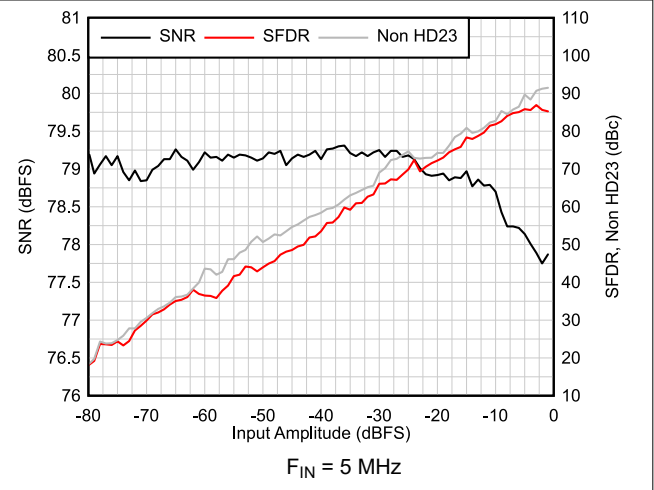
图 6-12. AC Performance vs Input Amplitude
