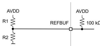
图 8-41. Configuration of external voltage on REFBUF pin
