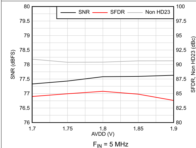
图 6-15. AC Performance vs AVDD
