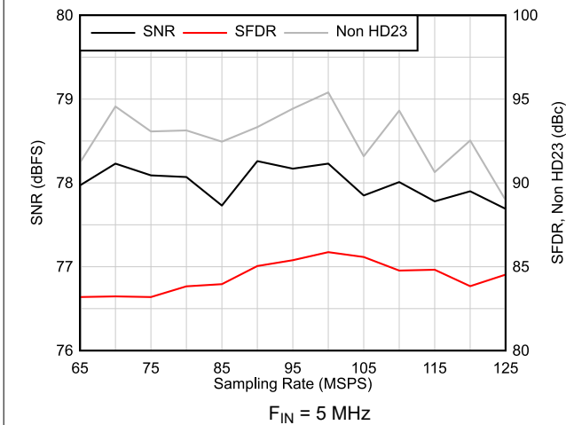
图 6-13. AC Performance vs Sampling Rate
