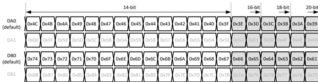
图 8-37. 1-wire output bit mapping
