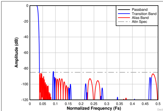
图 8-26. Decimation by 16 complex frequency response
