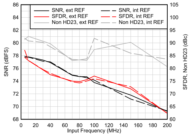
图 6-10. AC Performance vs Input Frequency
