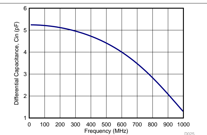
Figure 195. Differential Input Capacitance, C_{in}
