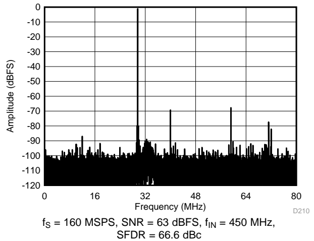
Figure 10. FFT for 450-MHz Input Signal (Dither Off)
