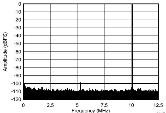
Figure 1. FFT for 10-MHz Input Signal (Dither On)
