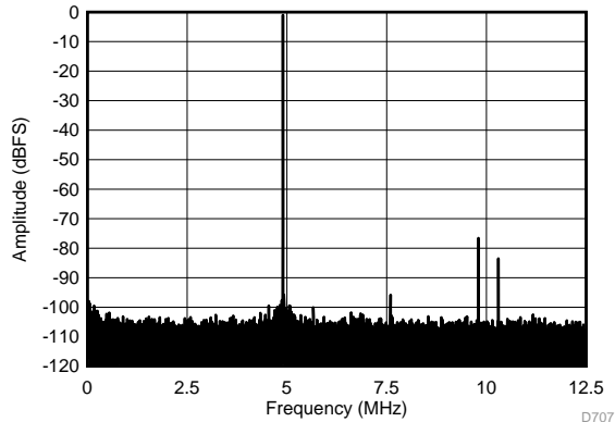
SFDR = 75.6 dBc, SNR = 69.8 dBFS, SINAD = 68.8 dBFS, THD = 74.8 dBc, HD2 = -75.6 dBc, HD3 = -82.5 dBc
