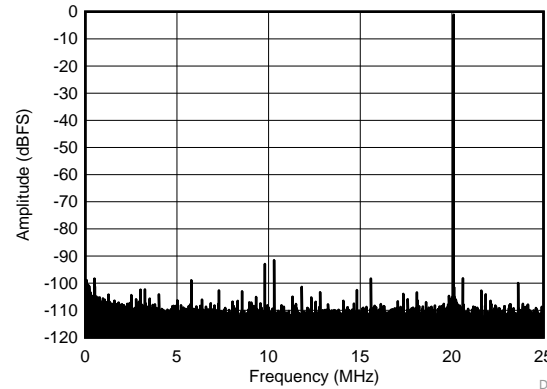
SFDR = 90.4 dBc, SFDR = 94.7 dBc (non 23), SNR = 73.9 dBFS, SINAD = 73.7 dBFS, THD = 87.5 dBc, HD2 = -91.9 dBc, HD3 = -90.4 dBc
