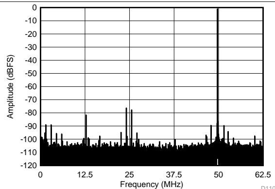
SFDR = 75.3 dBc, SNR = 69.1 dBFS, SINAD = 67.8 dBFS, THD = 72.7 dBc, HD2 = -76.7\text{ dBc} , HD3 = -75.3\text{ dBc}
