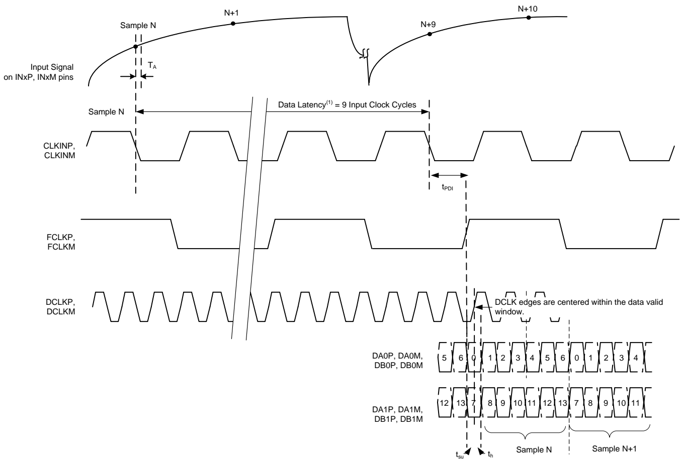
Figure 135. Latency Diagram
