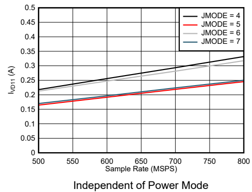
图 5-78. Quad Channel, I_{VD11} vs F_S for JMODES 4 - 7
