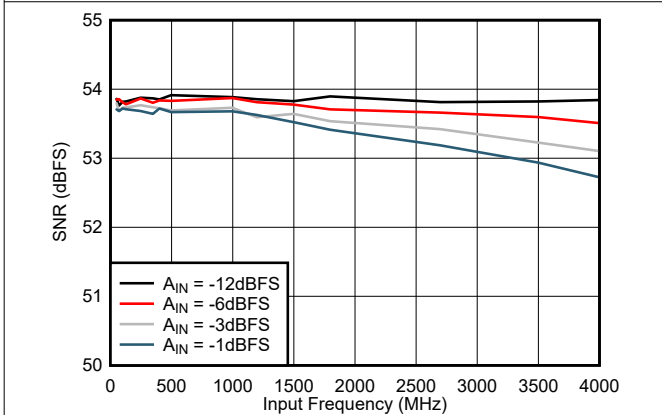
图 5-15. SNR vs Input Frequency
