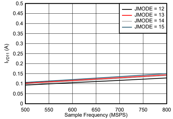
图 5-100. Single Channel, I_{VD11} vs F_S for JMODES 12 - 15
