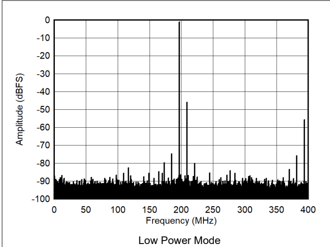
图 5-13. Single Tone FFT at 1797MHz and -1dBFS
