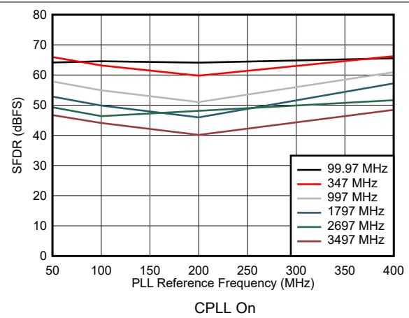
图 5-64. SFDR vs Reference Clock Frequency
