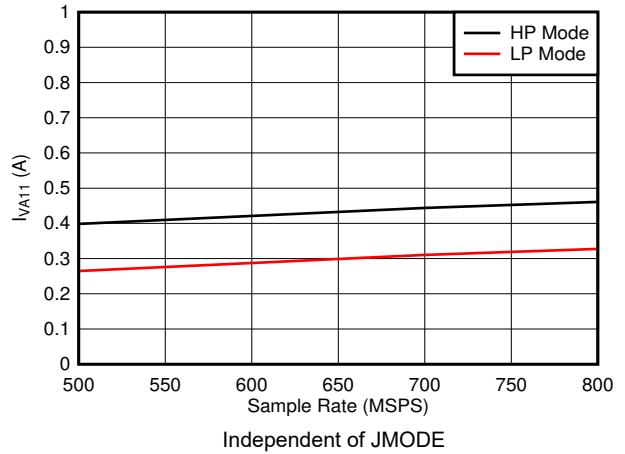
图 5-76. Quad Channel, I_{VA11} vs F_S
