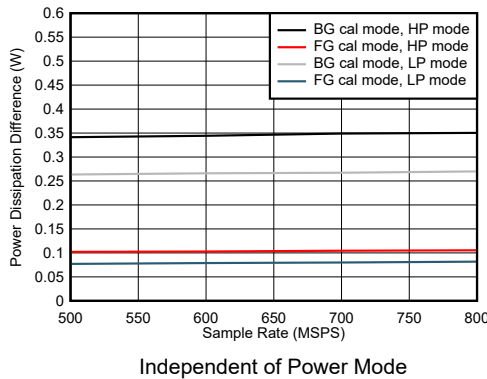
图 5-101. Quad Channel, Power Dissipation Change with Calibration Mode
