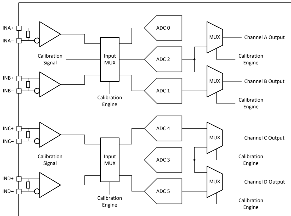
图 6-15. Quad Channel Calibration System Block Diagram
