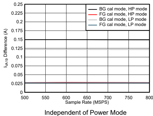
图 5-104. Quad Channel, I_{VA19} Change with Calibration Mode
