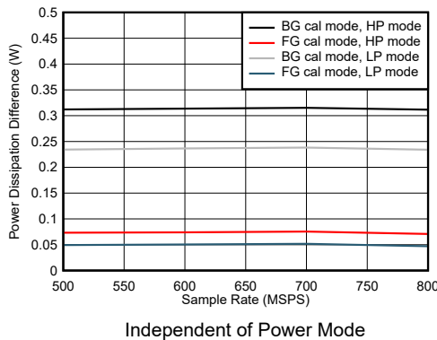
图 5-103. Single Channel, Power Dissipation Change with Calibration Mode
