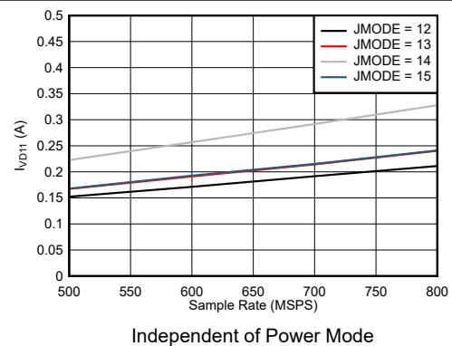
图 5-80. Quad Channel, I_{VD11} vs F_S for JMODES 12 - 15
