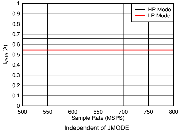
图 5-75. Quad Channel, I_{VA19} vs F_S
