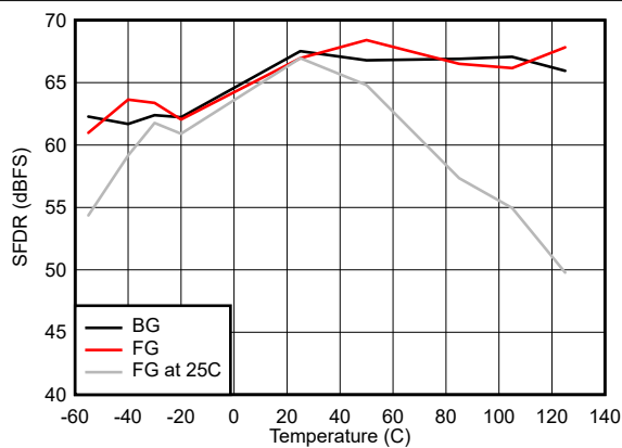
图 5-35. SFDR vs Temperature
