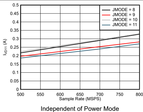
图 5-79. Quad Channel, I_{VD11} vs F_S for JMODES 8 - 11
