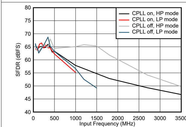
图 5-65. SFDR vs Input Frequency and CPLL and Power Mode
