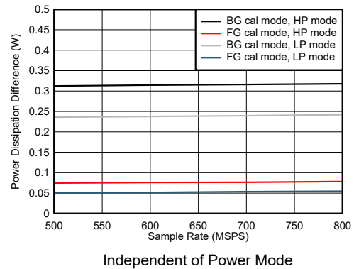
图 5-102. Dual Channel, Power Dissipation Change with Calibration Mode
