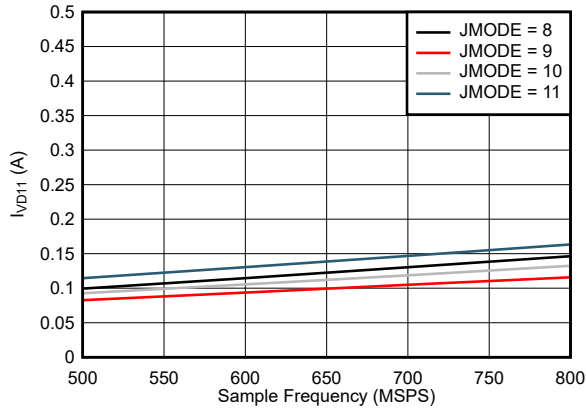
图 5-99. Single Channel, I_{VD11} vs F_S for JMODES 8 - 11
