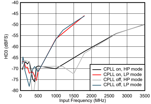
图 5-70. HD3 vs Input Frequency and CPLL and Power Mode
