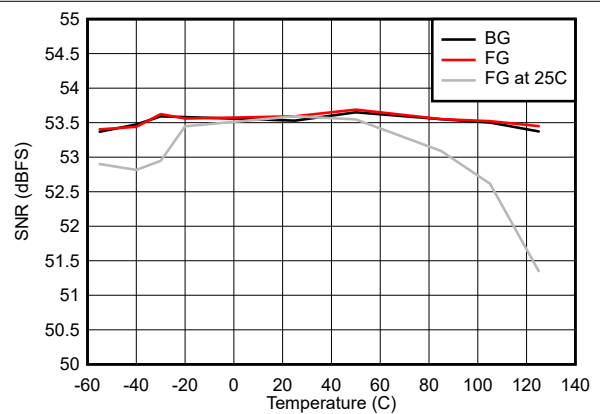
图 5-34. SNR vs Temperature
