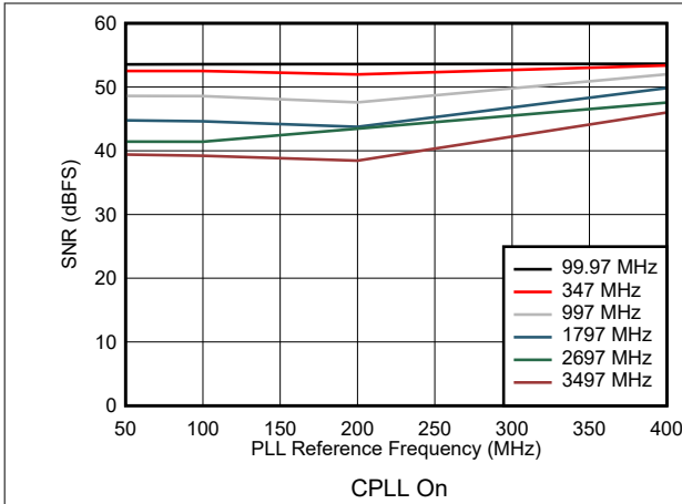
图 5-63. SNR vs Reference Clock Frequency
