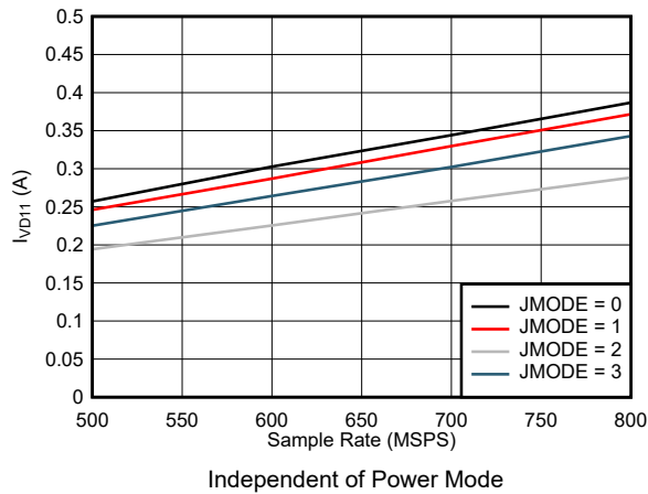
图 5-77. Quad Channel, I_{VD11} vs F_S for JMODES 0 - 3
