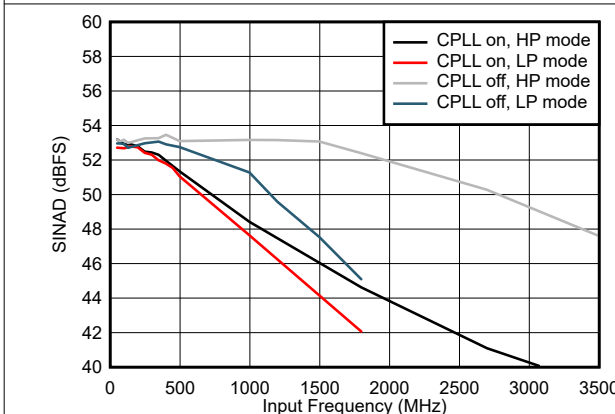
图 5-67. SINAD vs Input Frequency and CPLL and Power Mode
