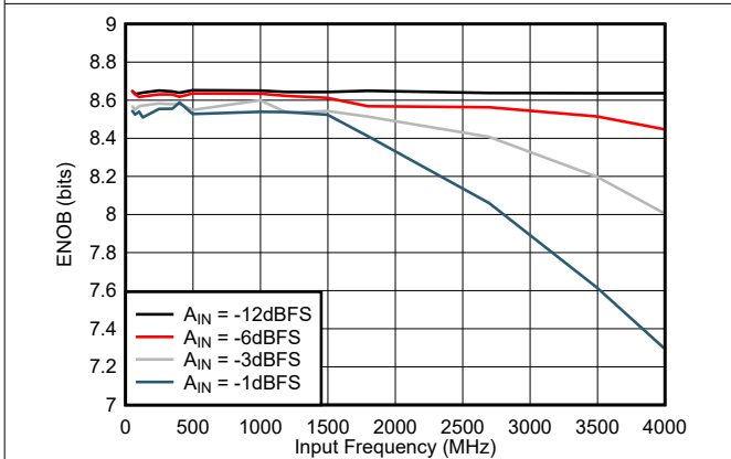
图 5-17. ENOB vs Input Frequency
