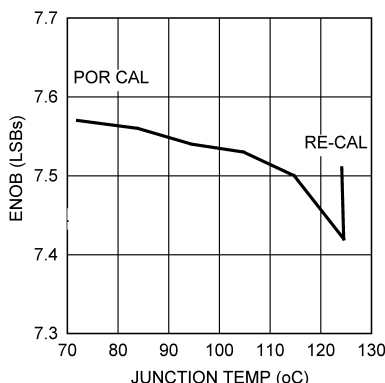
Figure 46. ENOB vs. Junction Temperature, 249 MHz Input
