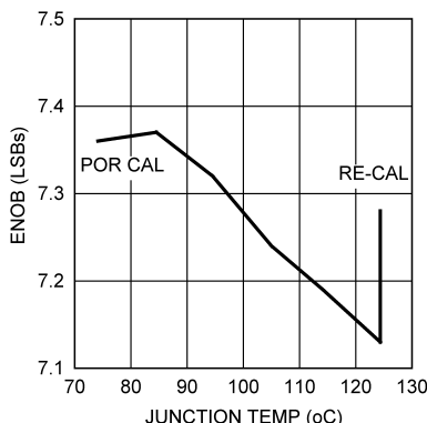
Figure 45. ENOB vs. Junction Temperature, 749 MHz Input
