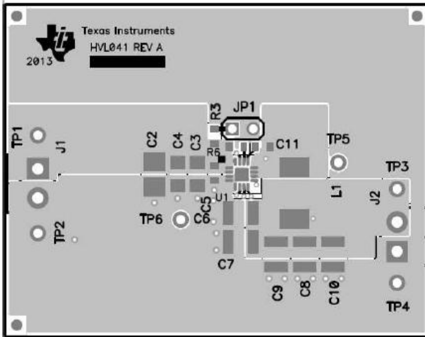
PMP10002_RevB: Top Side Assembly
