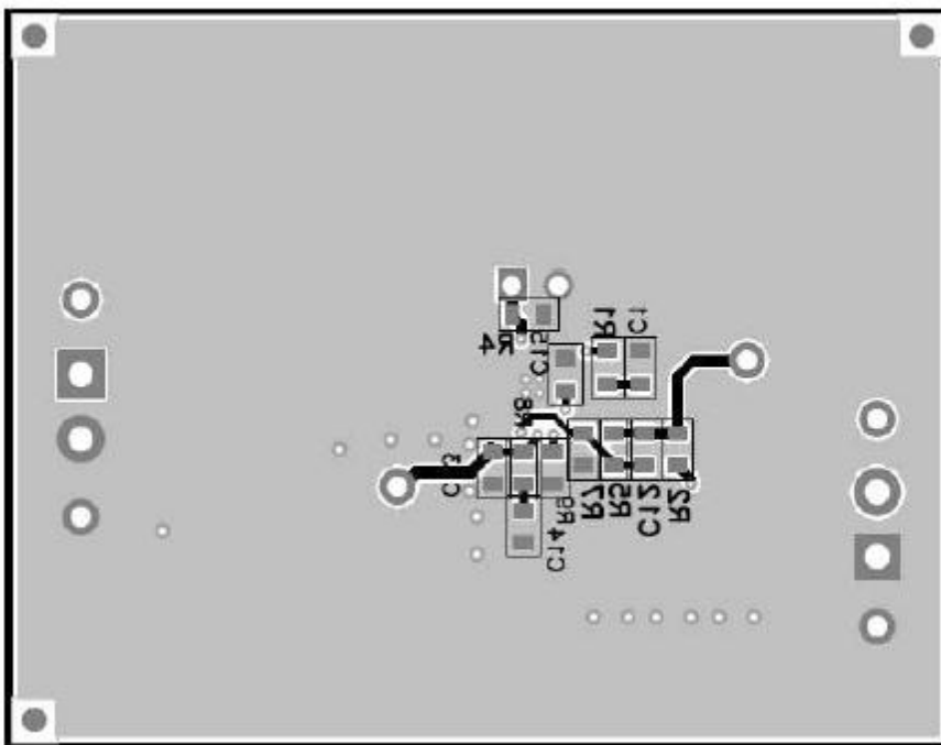
PMP10002_RevB: Bottom Side Assembly
