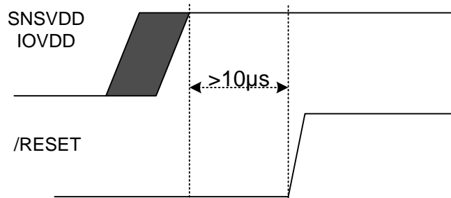
Figure 1-5 Suggested /RESET waveform during Power-On
