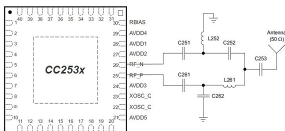
Figure 3. Discrete ref design for the CC253x
