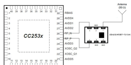
Figure 4. DEA202450BT- 210A1 for the CC253x
