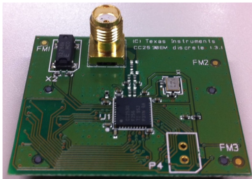
Figure 1. Photo of the discrete solution.
