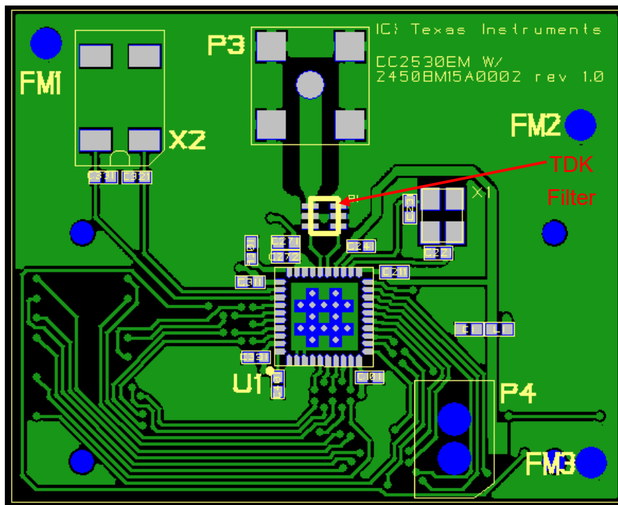
Figure 5. Texas Instruments CC2530 evaluation board with TDK DEA202450BT- 210A1
